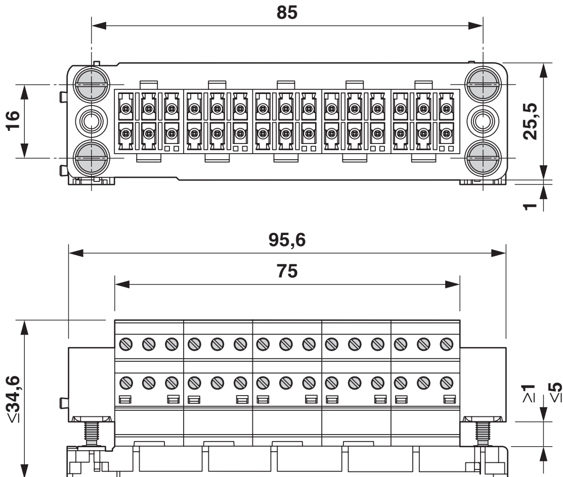
Dimensional drawing
