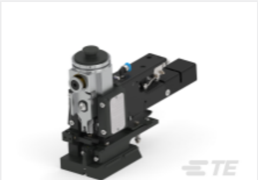
TE Part #2150719-1 OCEAN_2.0_Applicator-E-180F-REM
