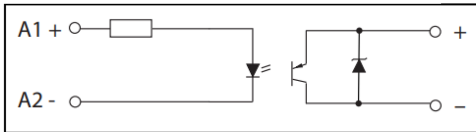
Simplified circuit diagram 8 A, 24 VDC version with bipolar Transistor Output
