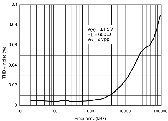
Figure 10. THD + noise vs. frequency
