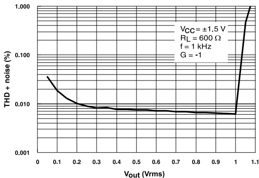
Figure 8. THD + noise vs. V_{out} , R_L = 600\ \Omega
