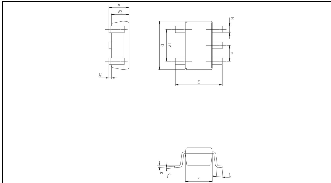
Figure 12. SOT23-5 package outline
