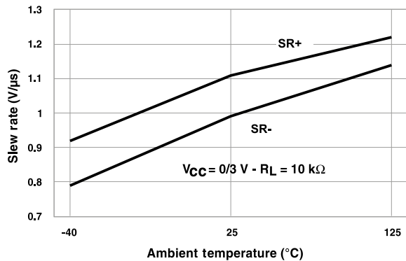
Figure 7. Slew rate vs. temperature
