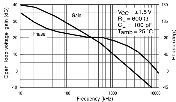
Figure 5. Voltage gain and phase vs. frequency, R_L = 600\text{ }\Omega , C_L = 100\text{ pF}
