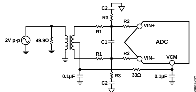
For baseband applications where SNR is a key parameter, differential transformer coupling is the recommended input configuration. An example is shown in Figure 48. To bias the analog input, the VCM voltage can be connected to the center tap of the secondary winding of the transformer.
