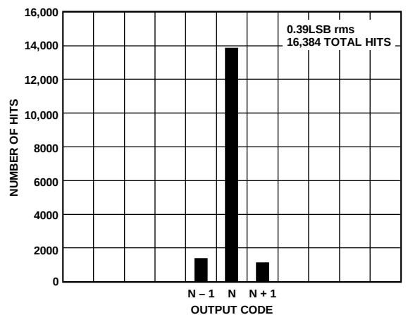
Figure 38. AD9613-250 Grounded Input Histogram
