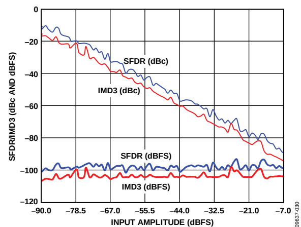
Figure 23. AD9613-210 Two-Tone SFDR/IMD3 vs. Input Amplitude ( A_{IN} ) with f_{IN1} = 184.12 , f_{IN2} = 187.12 MHz, f_s = 210 MSPS
