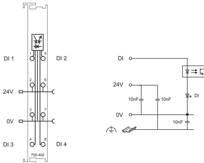
Fig. 2.1.1-3: 4-Channel Digital Input Module 750-402
