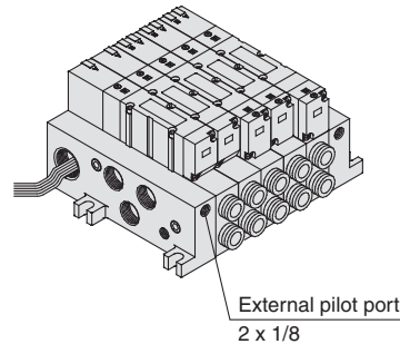
<Manifold>
