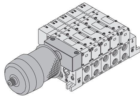
Plug lead type
