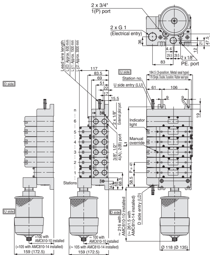
Plug-in type
