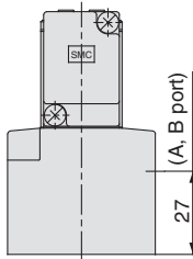
Bottom ported drawing
