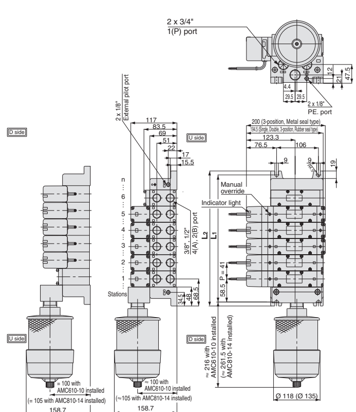
Plug lead type
