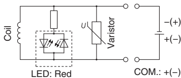
DC: Single
