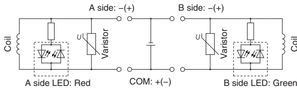
DC: Double
