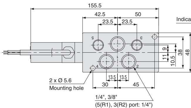
Bottom ported drawing
