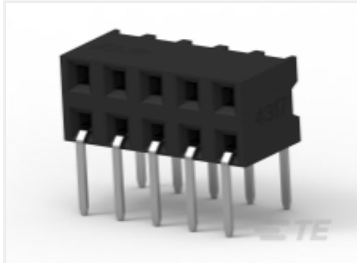
TE Part # 1-2314925-4 14P,2MM,B-B,REC,DRHZ,2.8,0.38AU,TR
