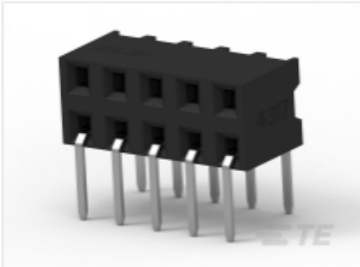
TE Part # 1-2307718-4 14P,2MM,B-B,REC,DRHZ,2.1,0.38AU,TR
