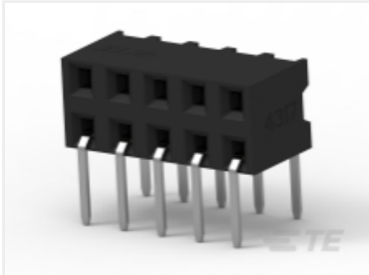
TE Part # 1-2307720-4 14P,2MM,B-B,REC,DRHZ,3.4,0.38AU,TUBE
