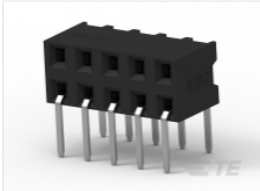
TE Part # 1-2314917-4 14P,2MM,B-B,REC,DRHZ,2.1,0.38AU,TB
