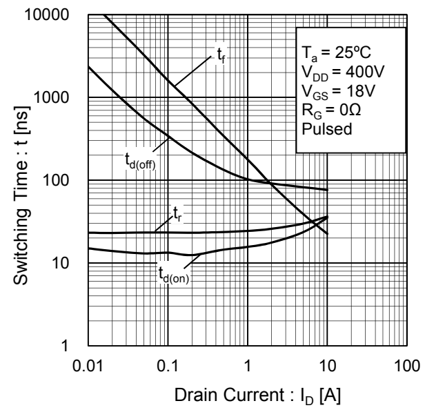
Fig.17 Switching Characteristics
