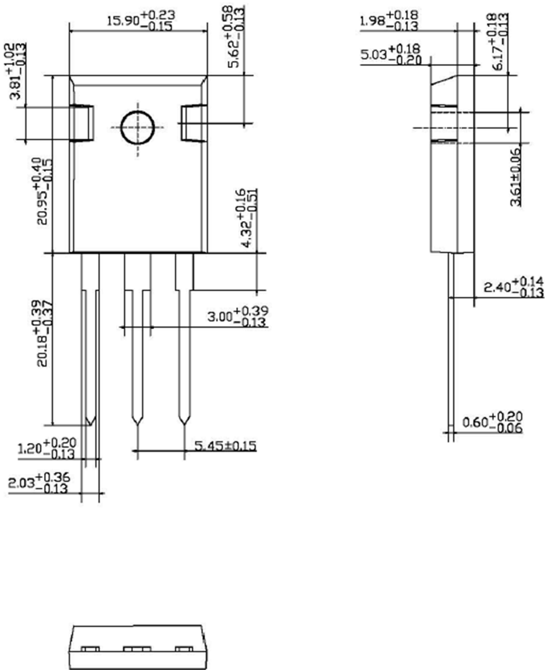
TO-247
