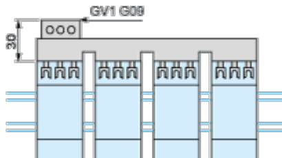
Sets of Busbars for GV2L and GV2LE Sets of busbars GV2G... with terminal block GV1G09
