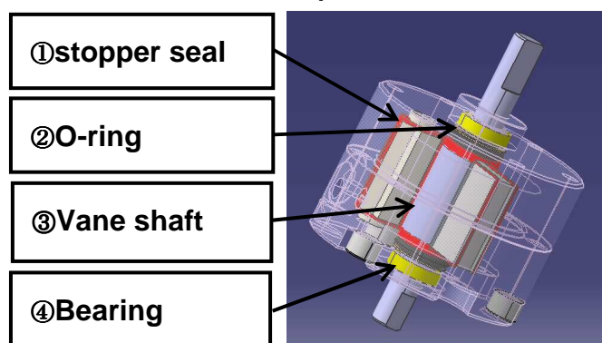
Fig 1.Vane type / Rotary actuator
