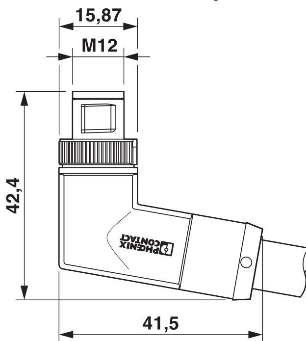
Dimensional drawing
