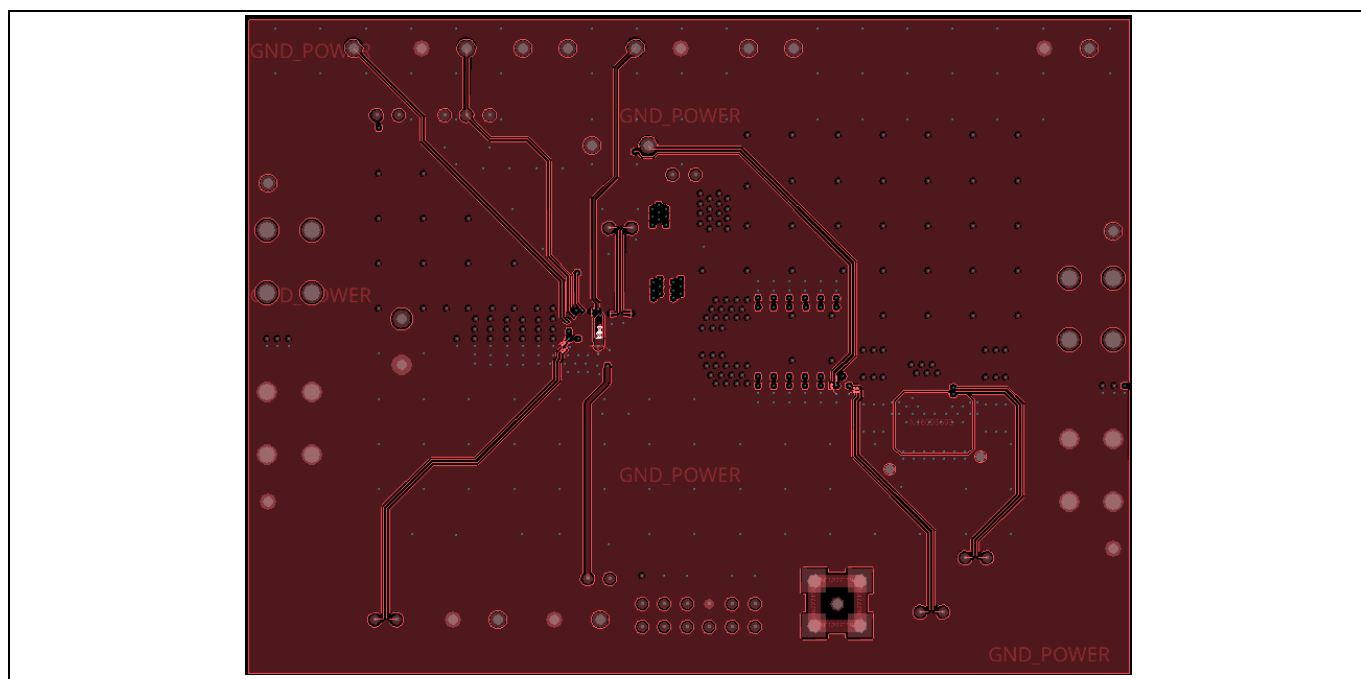
Figure 5 Inner layer 2
