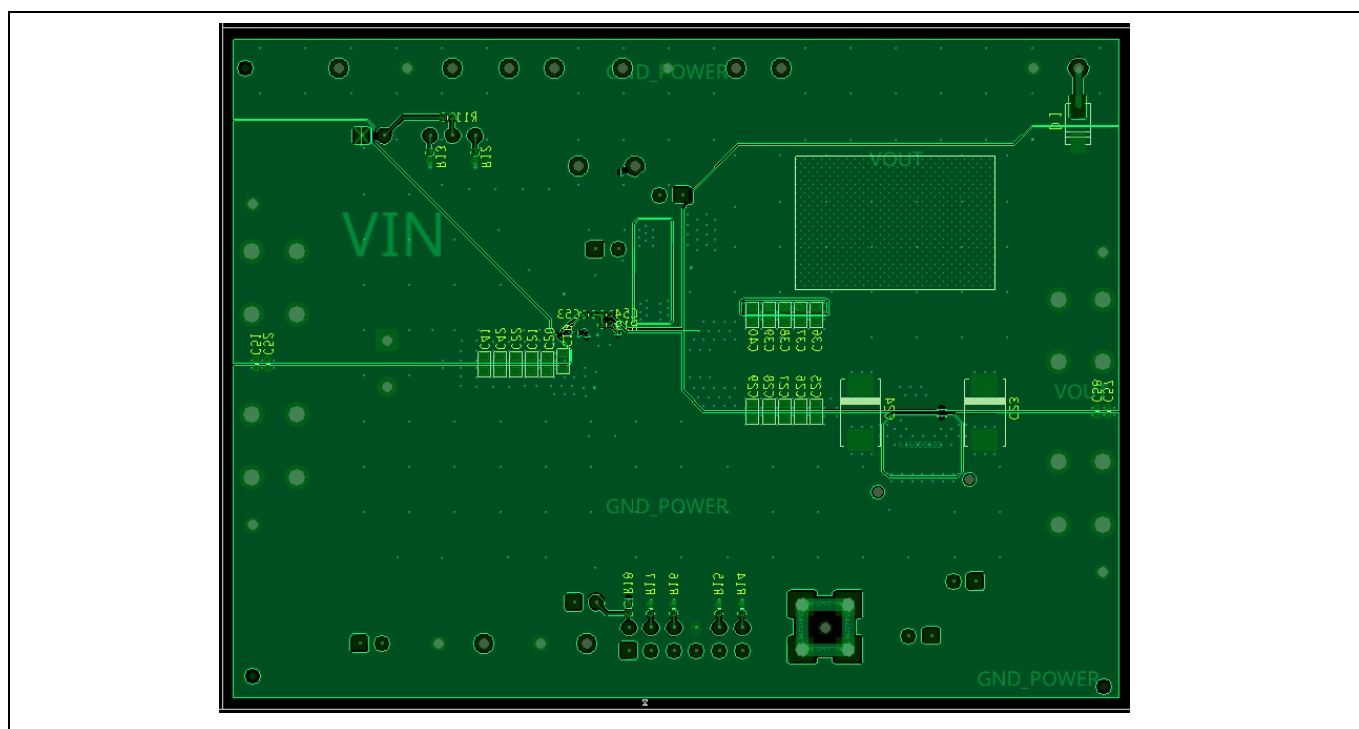
Figure 3 Bottom layer
