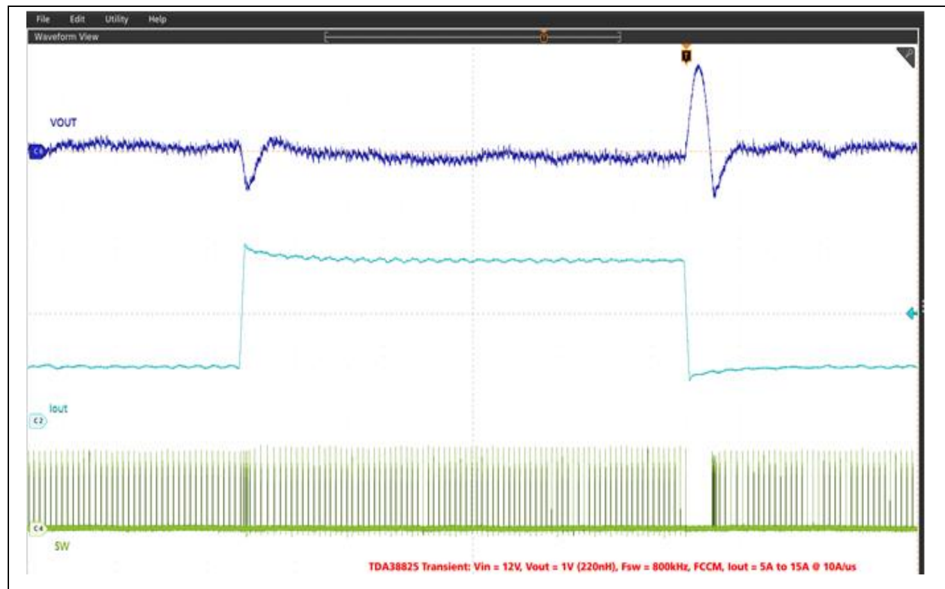
Figure 17 Transient response at 10 A step load current at 10 A/ \mu s slew rate: I_{OUT} = 5 A – 15 A, (Ch6: V_{OUT} , Ch2: I_{OUT} , Ch4: SW ), pk-pk: 55 mV, F_{SW} = 800 kHz
