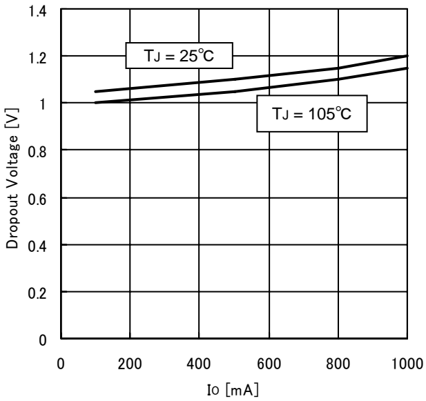
Figure 3. Dropout voltage
