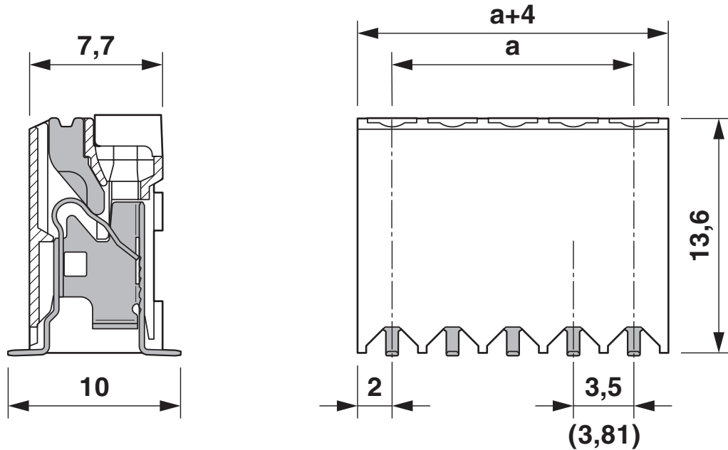
Dimensional drawing
