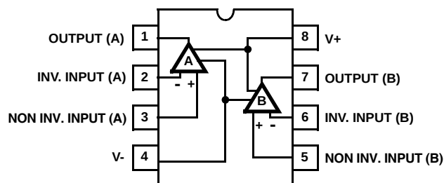
CA3260, CA3260A (8 LD PDIP) TOP VIEW
