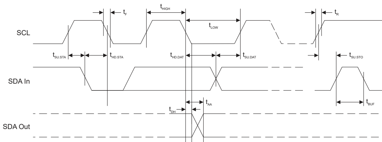
Figure 4-1. Bus Timing
