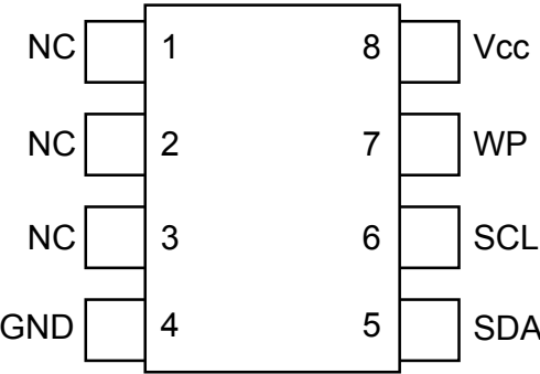
8-Lead PDIP/SOIC/TSSOP (Top View)
