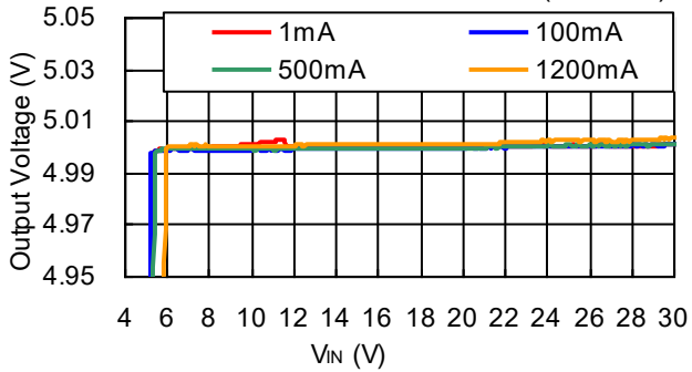
R1245x00xC/R1245x00xD V OUT =5.0V
