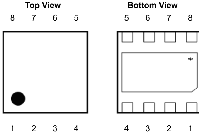
DFN(PL)2020-8 Pin Configuration
