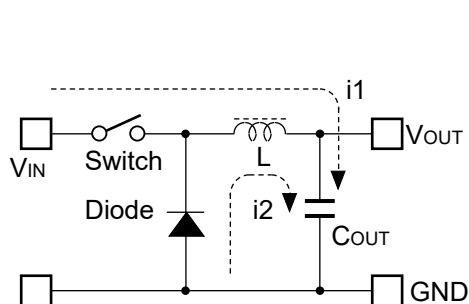
Basic Circuit
