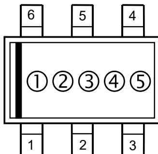
SOT-23-6W Part Markings
