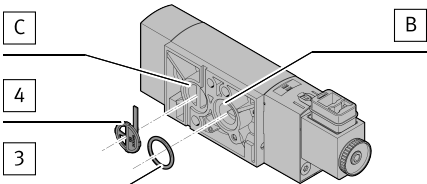
Fig. 2 Valve function 5/2
