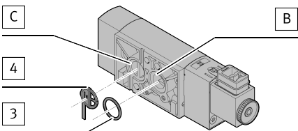
Fig. 3 Valve function 3/2
