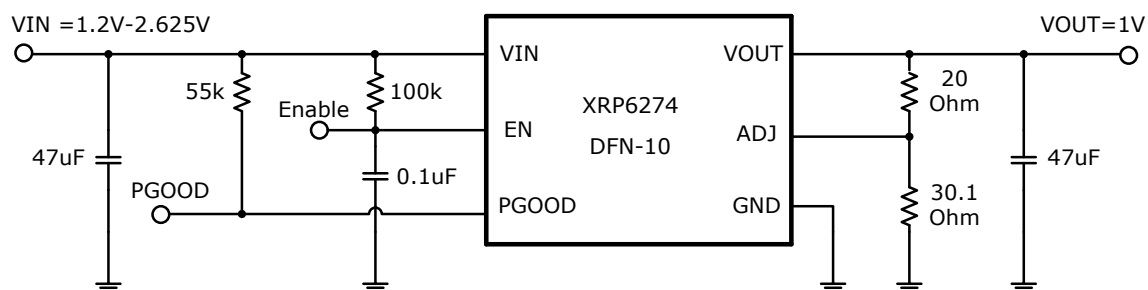
Fig. 14: XRP6274 Typical Application Diagram
