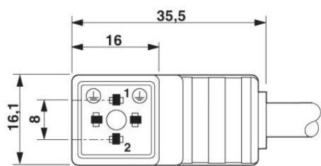
Valve connector, type C
