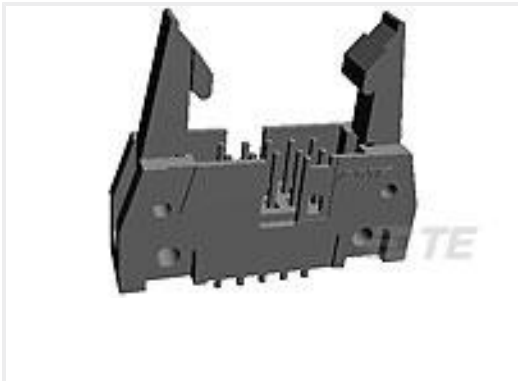
TE Part #5499160-2 A/L UNIV HDR 14P VERT SHT LAT
