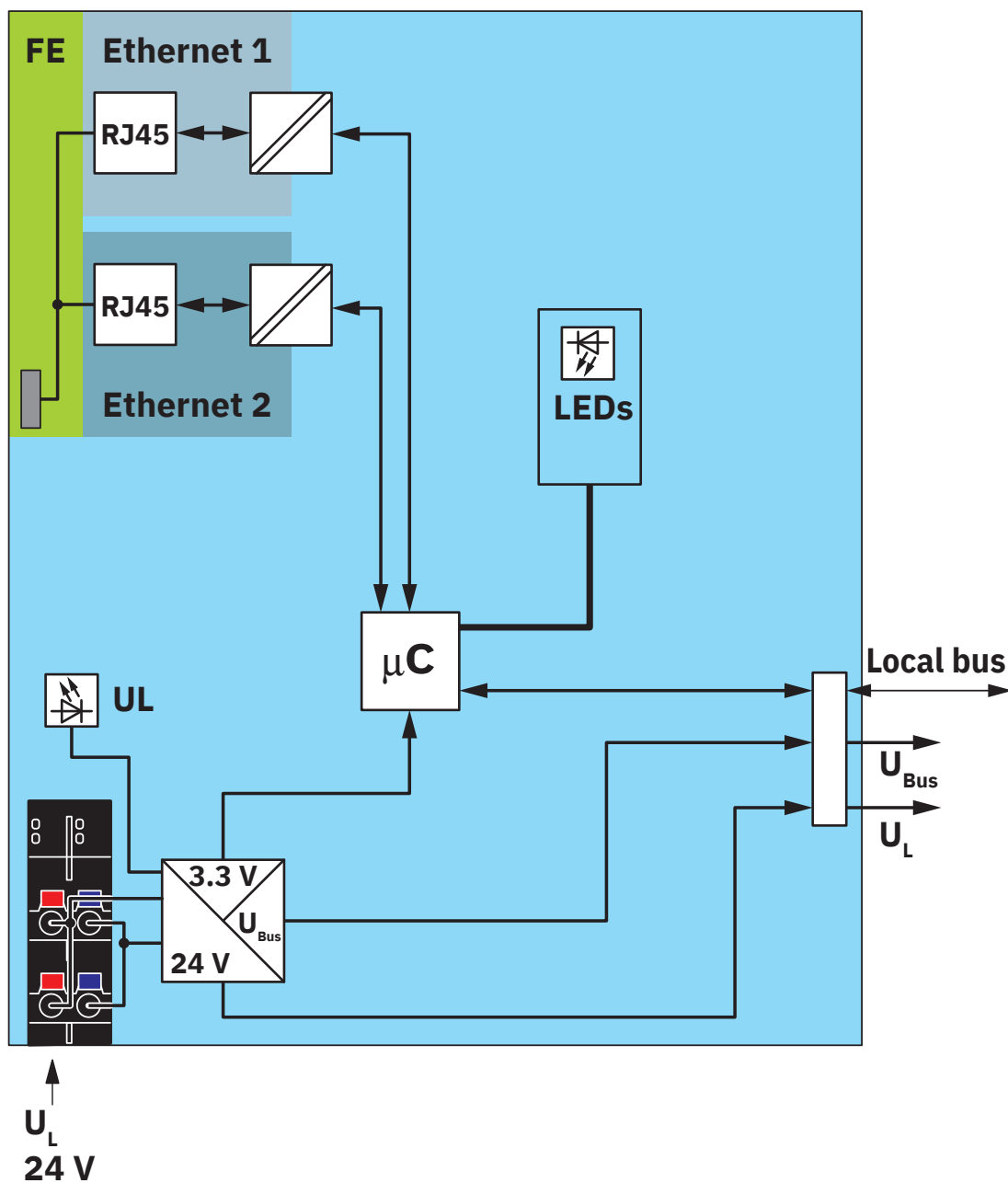
Block diagram
