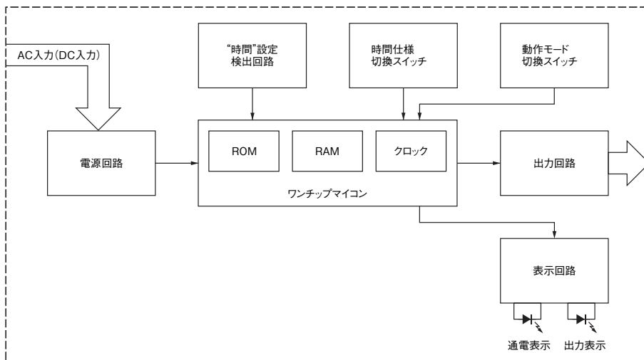
形H3DK-S1/-S2
