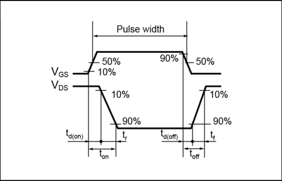
Fig.1-2 Switching Waveforms
