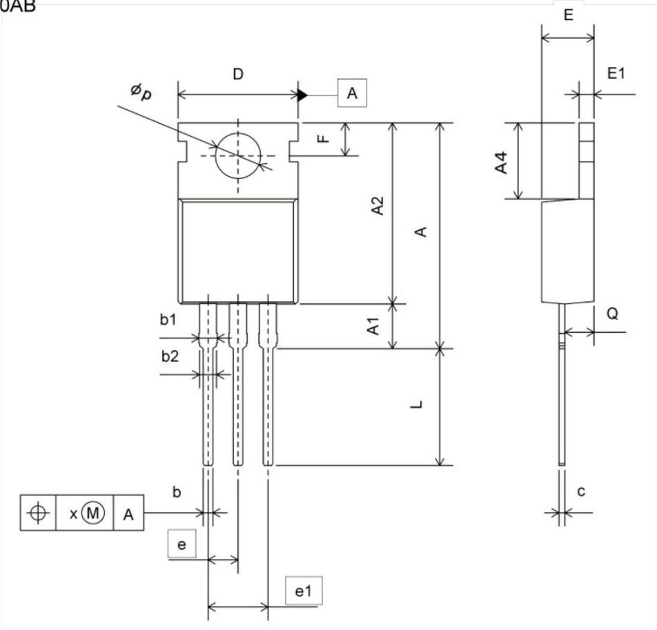
TO-220AB
