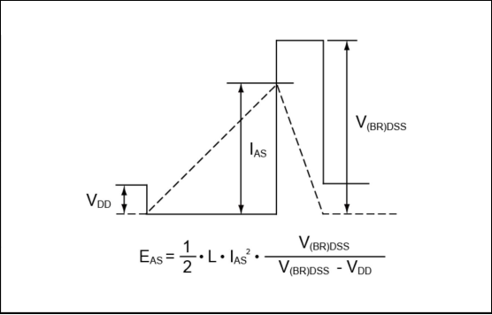
Fig.3-2 Avalanche Waveform
