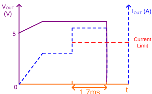
Figure 8: Over-Current Limit
