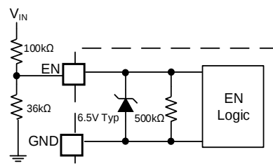
Figure 2: Zener Diode (6.5V Typical)
