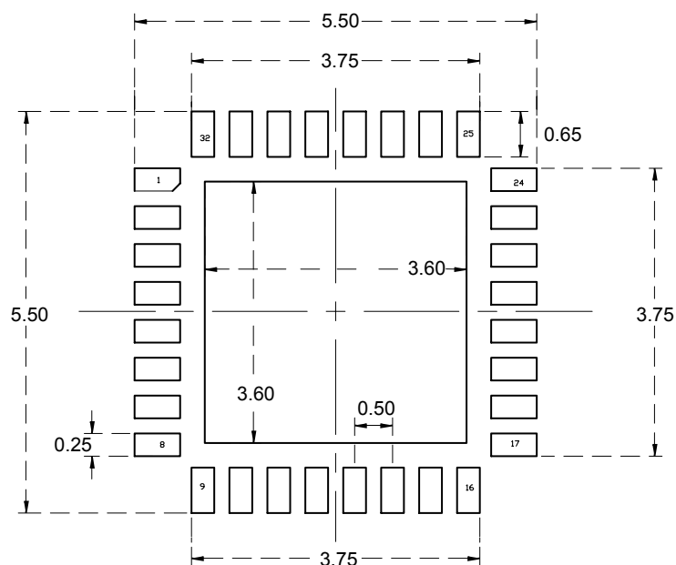
Figure 20. UFQFPN32 - Footprint example
