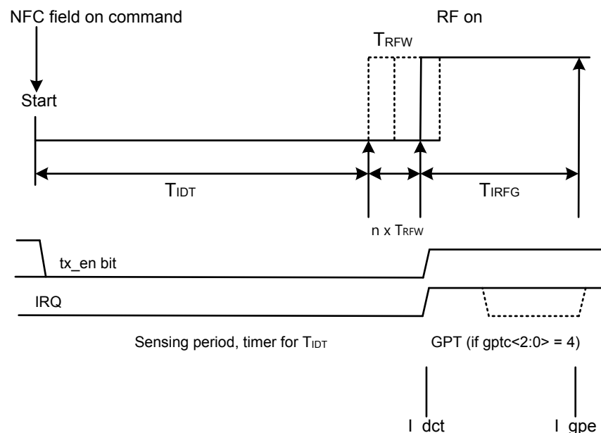
Figure 16. Direct command NFC field on (no RF collision)
