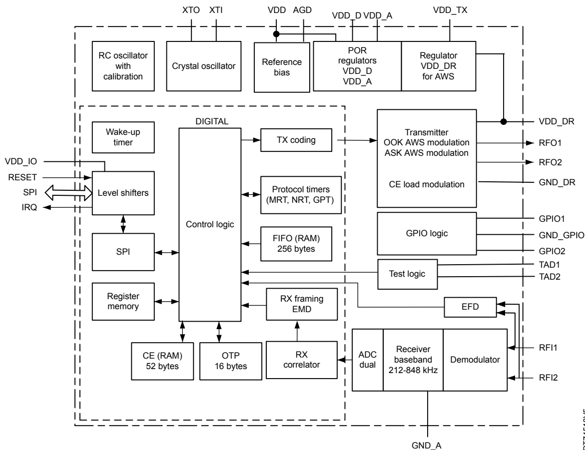
Figure 1. ST25R301 block diagram
