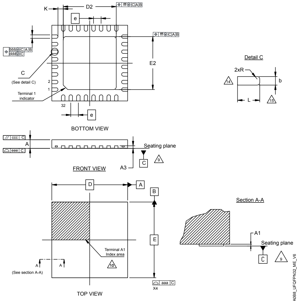
Figure 19. UFQFPN32 - Outline
