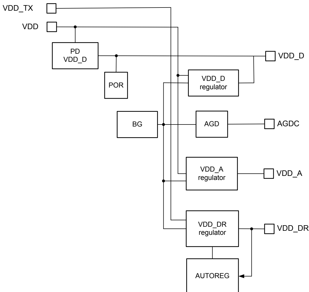
Figure 6. Power supply system
