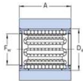
LUHR With double lip seal
