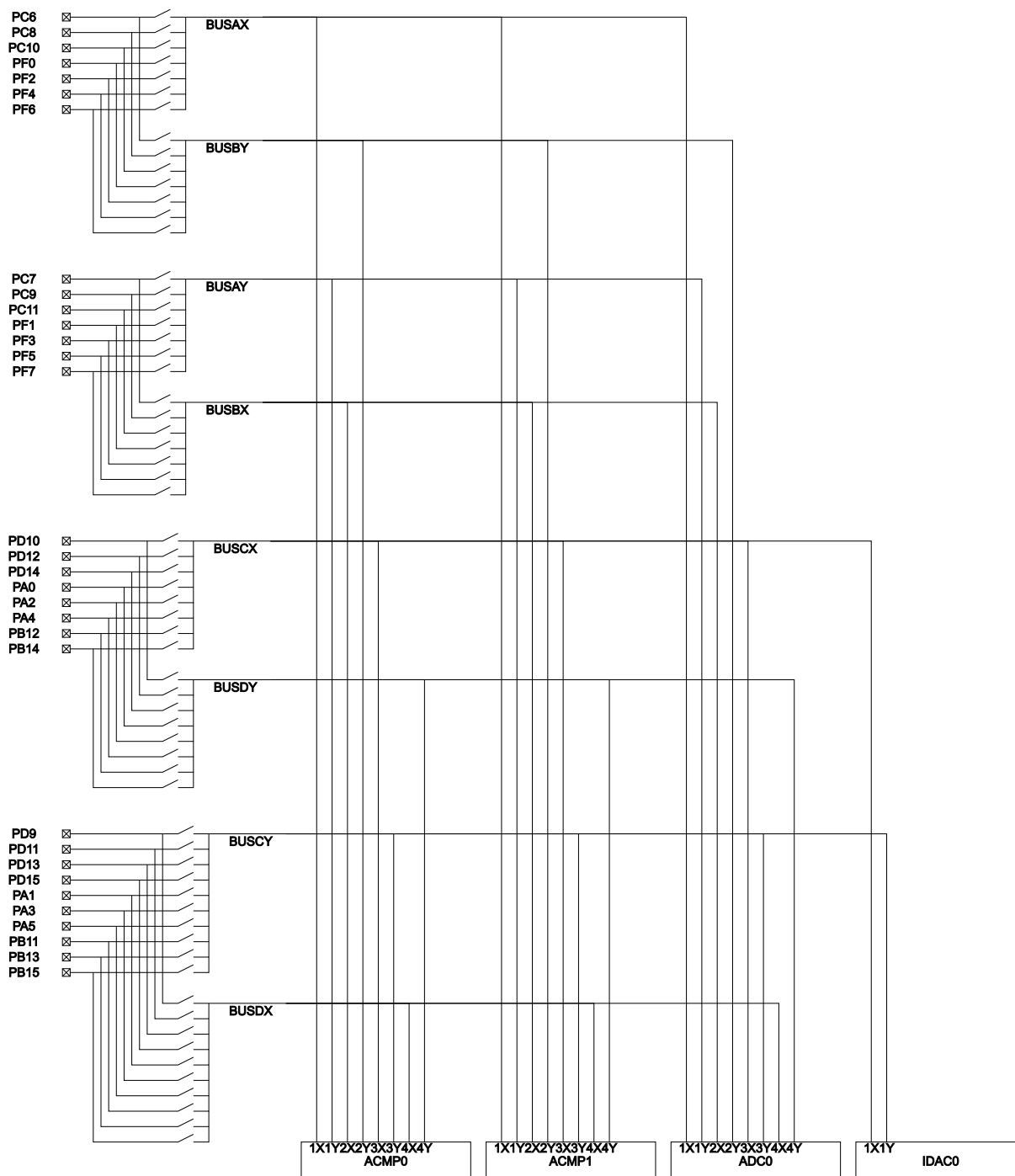
Figure 6.6. EFR32FG1 APORT
