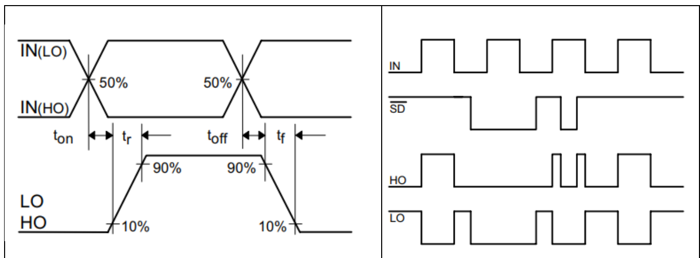
Figure 3 Switching timing diagram
