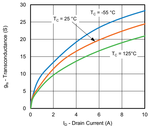
Transconductance
