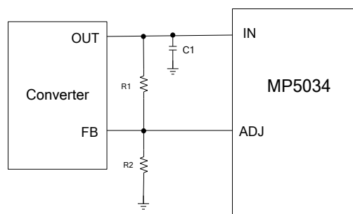
Figure 3: ADJ Configure
