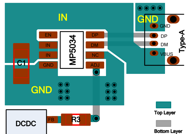
Figure 6: Recommended Layout
