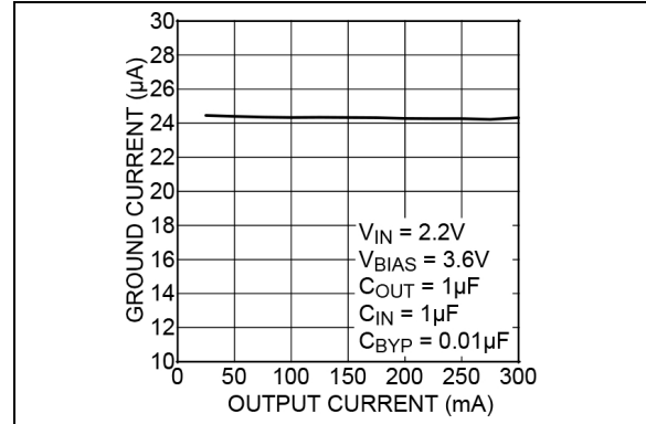
FIGURE 2-6: Ground Current (Total) vs. Output Current.
