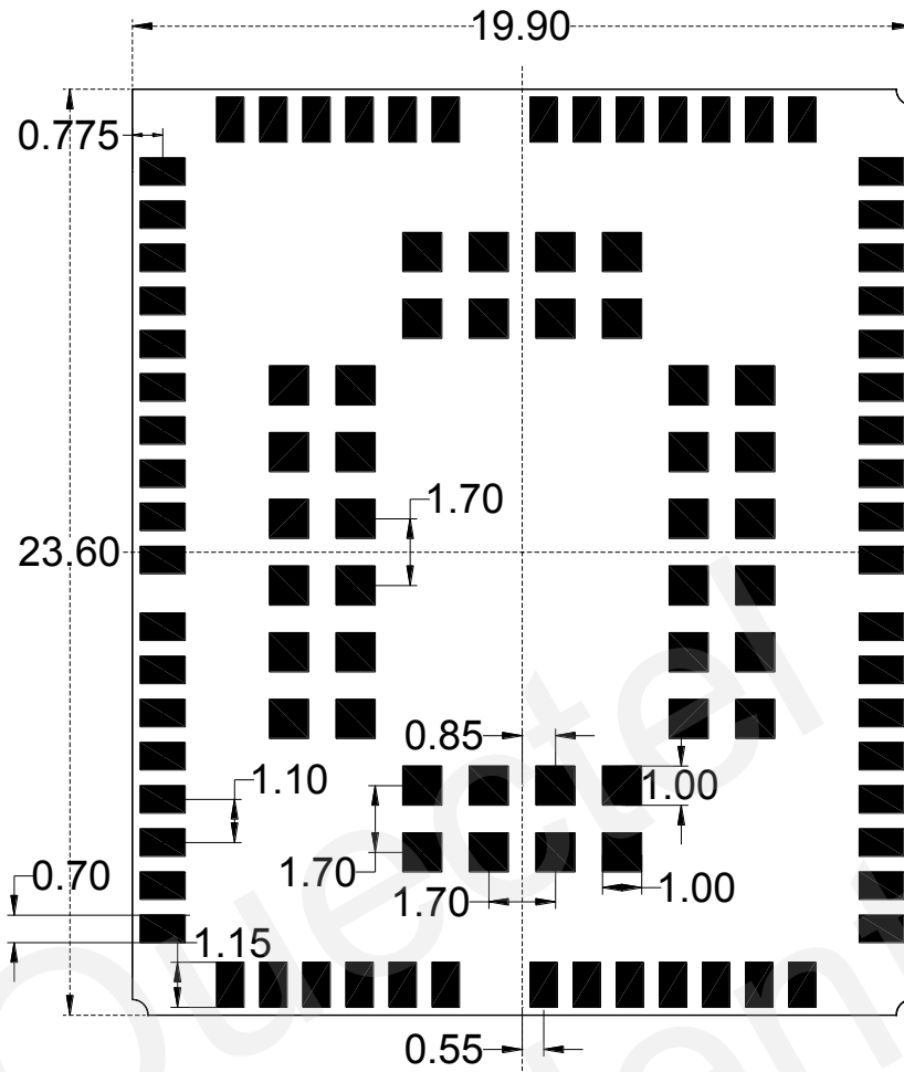
Figure 36: UG95 Bottom Dimension (Top View)
