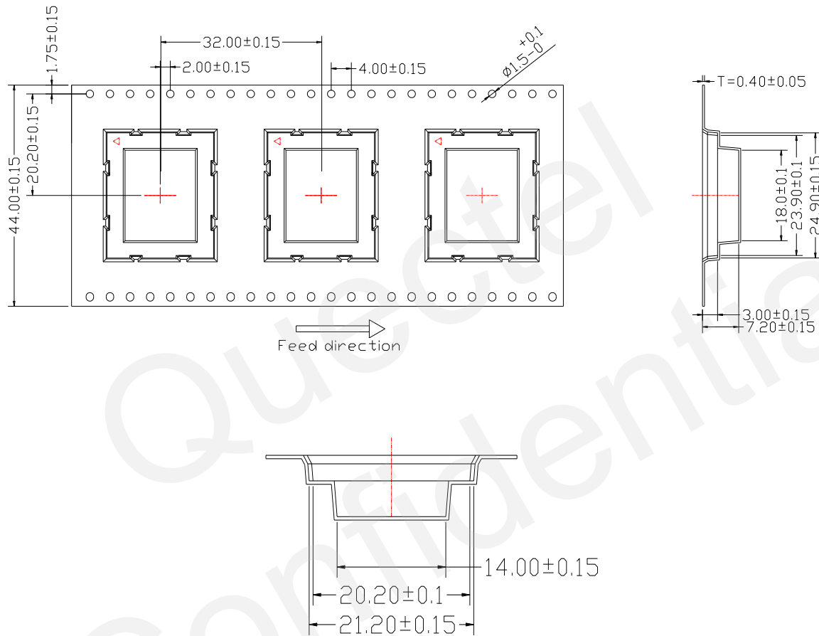
Figure 42: Tape and Reel Specification
