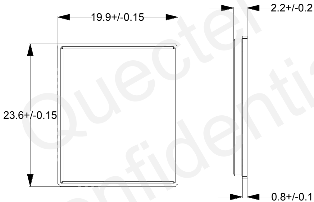
Figure 35: UG95 Top and Side Dimensions
