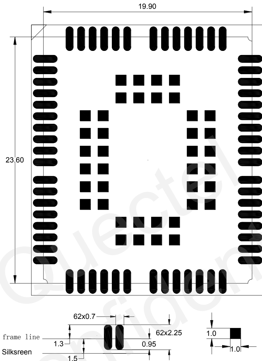
Figure 38: Recommended Stencil of UG95 (Top View)
