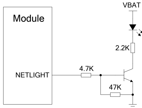
Figure 29: Reference Circuit of the NETLIGHT
