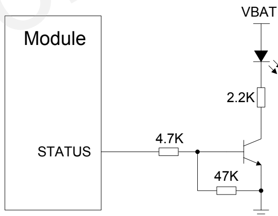
Figure 30: Reference Circuit of the STATUS
