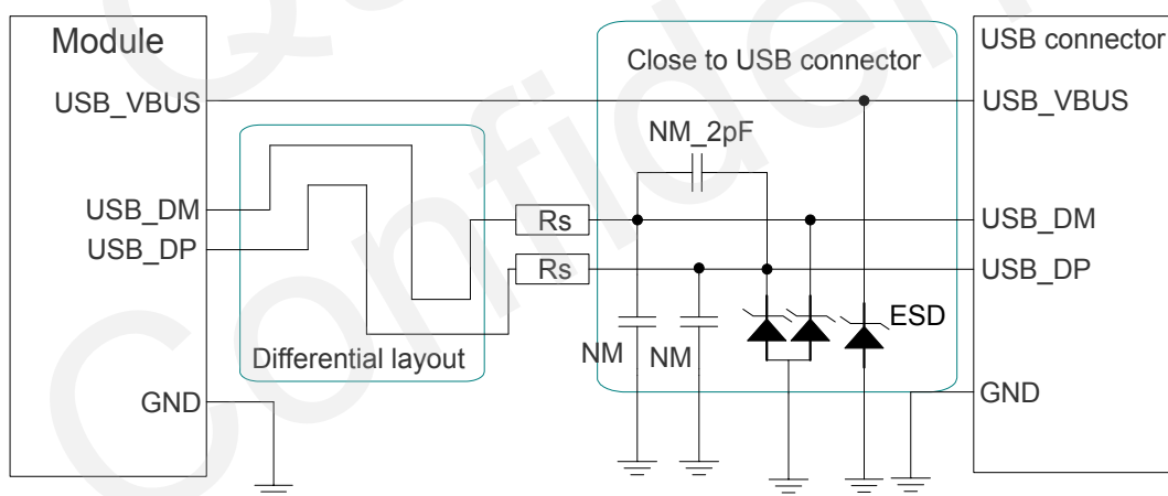
Figure 25: Reference Circuit of USB Application
