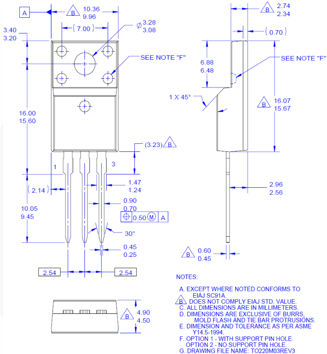
Figure 19. TO-220F 3L - TO220, MOLDED, 3LD, FULL PACK, EIAJ SC91, STRAIGHT LEAD
