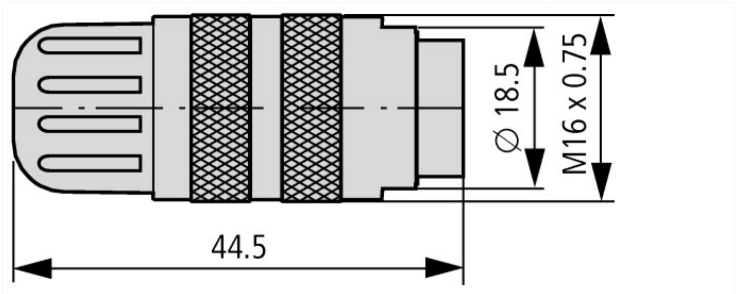
Plug connectors for SmartWire-DT round cables, flat
