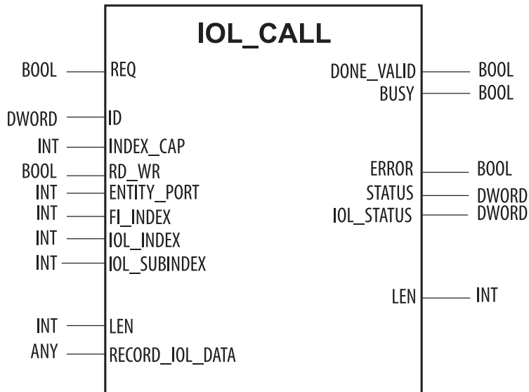
Fig. 32: IOL_CALL in accordance with IO-Link specification
