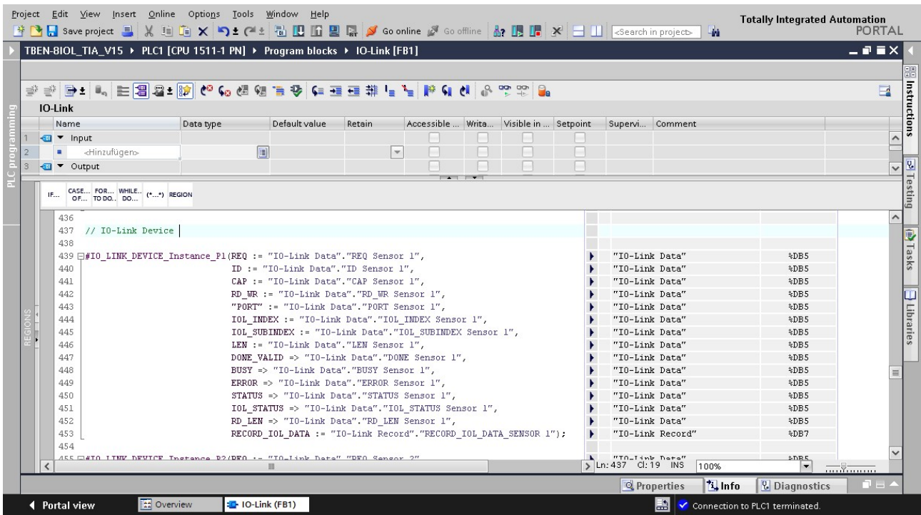
Fig. 40: Example call of Siemens FB "IO_LINK_DEVICE"
