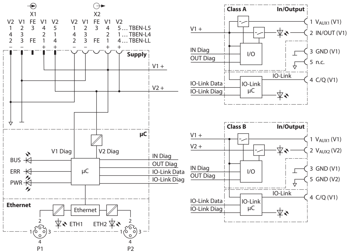
Fig. 5: Block diagram
