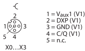
Fig. 18: Pin assignment of IO-Link master ports, Class A, X0...X3
