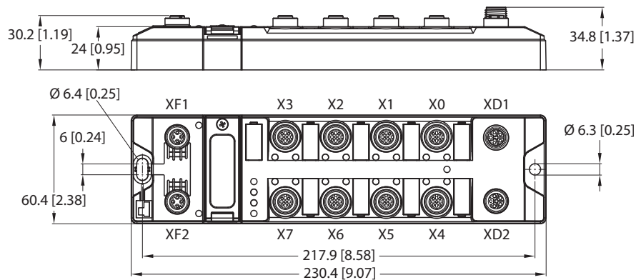
Fig. 4: Dimensions TBEN-LL-8IOL
