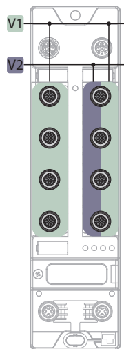
Fig. 16: Power supply of TBEN-LL-8IOL
