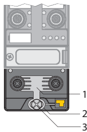
Fig. 9: Grounding clamp (1)
