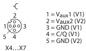
Fig. 19: Pin assignment of IO-Link master ports, Class B, X4...X7
