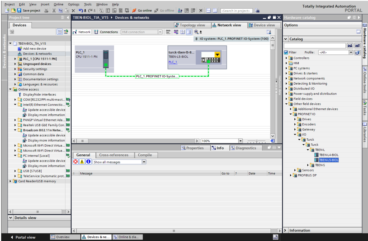
Fig. 34: Connecting the device to the PLC
