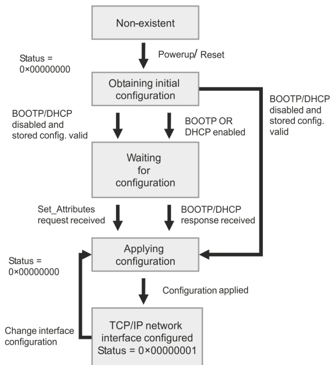
Fig. 49: TCP/IP object state diagram (acc. to CIP Spec., Vol.2, Rev. 1.1)
