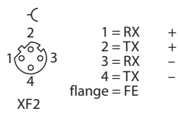
Fig. 13: Pin assignment Ethernet connectors
