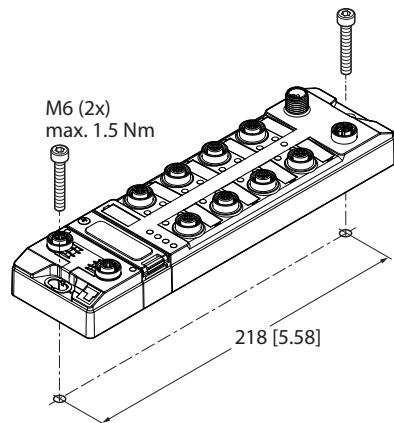
Fig. 6: Mounting the device on a mounting plate
