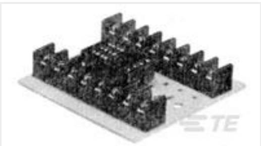
TE Part #1393837-1 27E460=SOCKET,R10,2POLE,PCB, TRCK-MNT,SCRW
