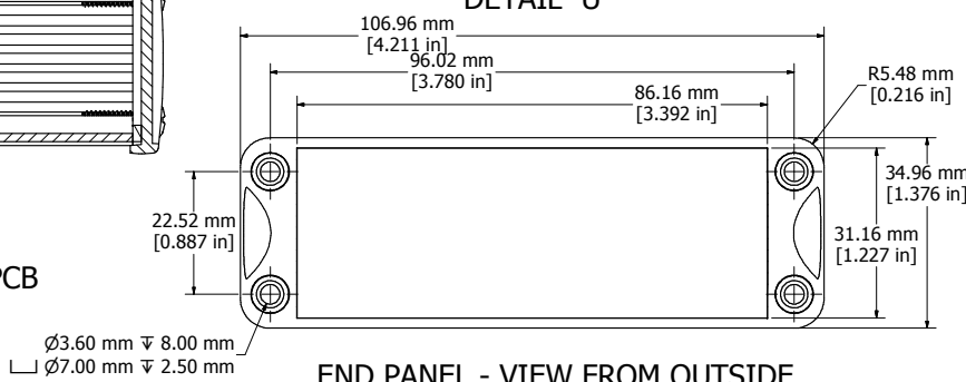
END PANEL - VIEW FROM OUTSIDE
