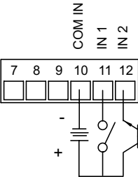
Sourcing Input
