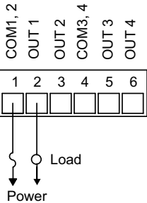
Relay Version
