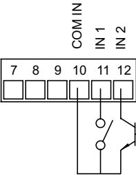
Sinking Input
