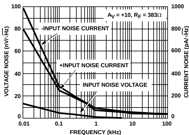
FIGURE 25. INPUT NOISE CHARACTERISTICS
