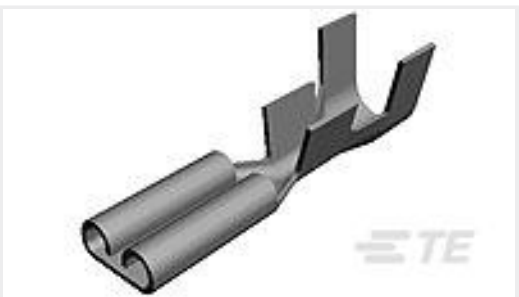
TE Part #160534-1 110 FASTON,REC.,17-20 AWG,BR
