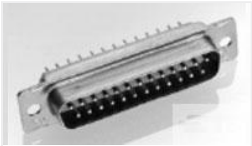
TE Part #205561-2 RECEPT ASSY,37 POSN,AMPLIMITE
