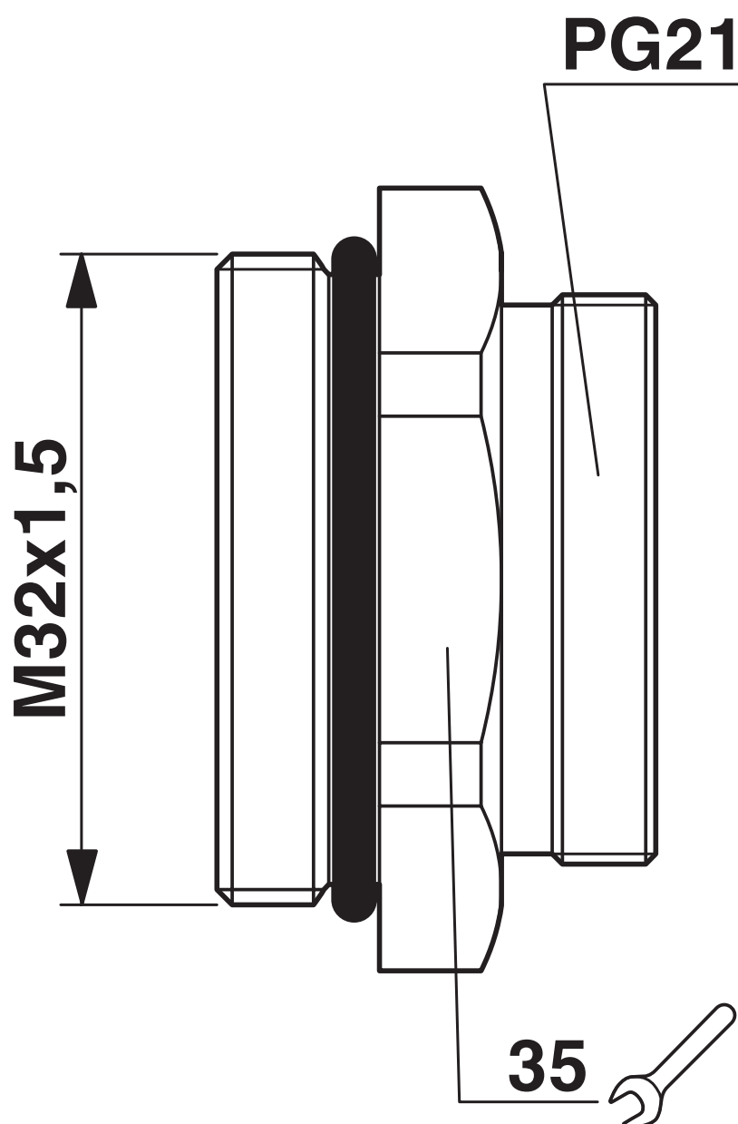
Dimensional drawing
