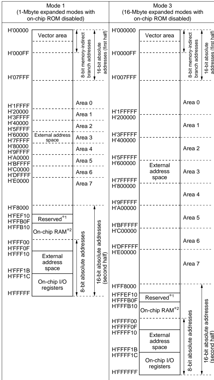
Figure 3.3 H8/307 Memory Map in Each Operating Mode (1)
