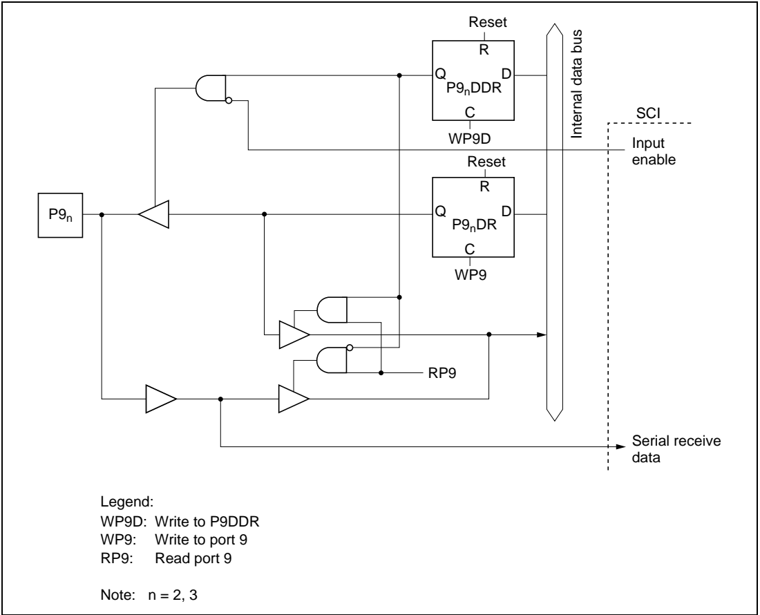
Figure C.8 (c) Port 9 Block Diagram (Pin P9_n , P9_n )
