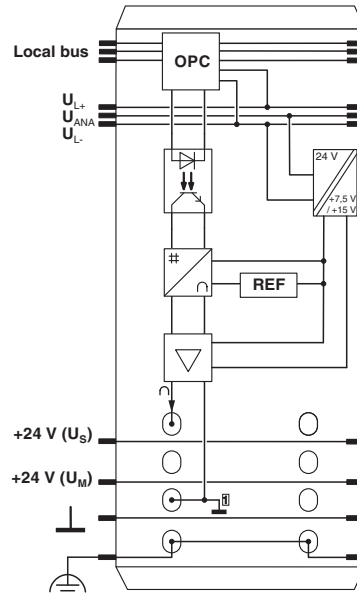
Block diagram
