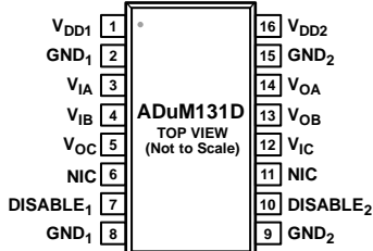
Figure 8. ADuM131D Pin Configuration
