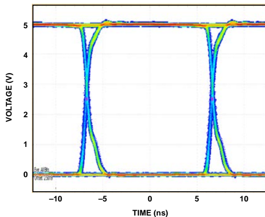
Figure 20. Eye Diagram
