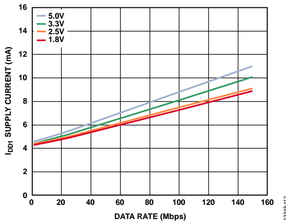
Figure 12. ADuM131D/ADuM131E I_{DD1} Supply Current vs. Data Rate at Various Voltages
