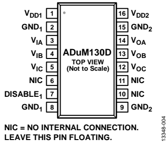
Figure 6. ADuM130D Pin Configuration
