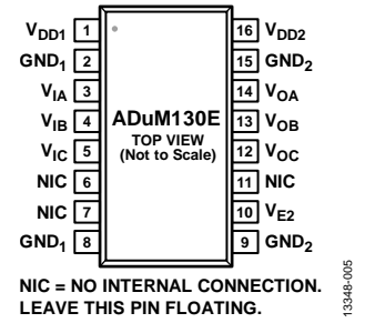
Figure 7. ADuM130E Pin Configuration
