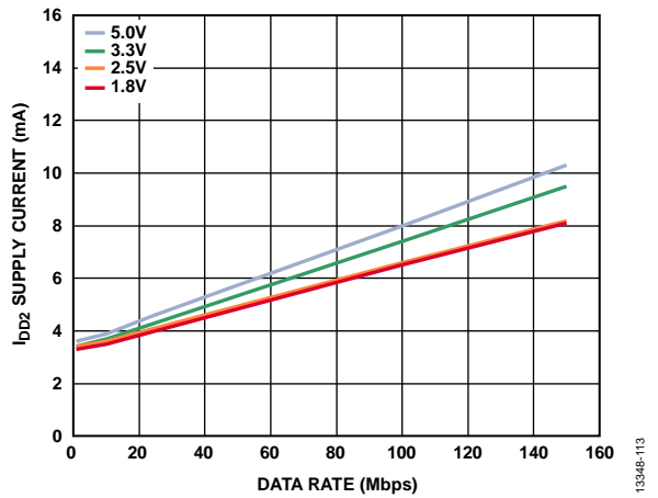
Figure 13. ADuM131D/ADuM131E I_{DD2} Supply Current vs. Data Rate at Various Voltages
