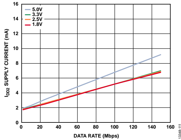
Figure 11. ADuM130D/ADuM130E I_{DD2} Supply Current vs. Data Rate at Various Voltages
