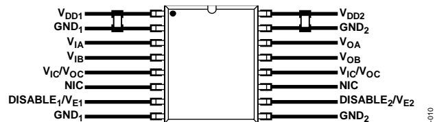
Figure 16. Recommended PCB Layout
