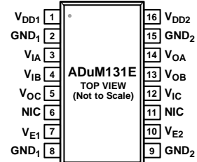
Figure 9. ADuM131E Pin Configuration
