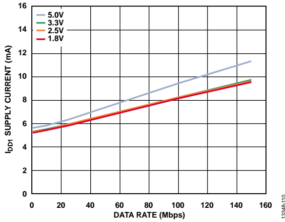
Figure 10. ADuM130D/ADuM130E I_{DD1} Supply Current vs. Data Rate at Various Voltages
