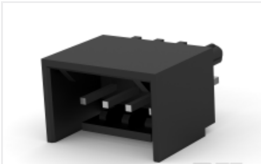
TE Part #CAT-104MTA-PVSHH Polyester Vertical PCB Header: 2.54 mm, Shrouded, MTA 100
