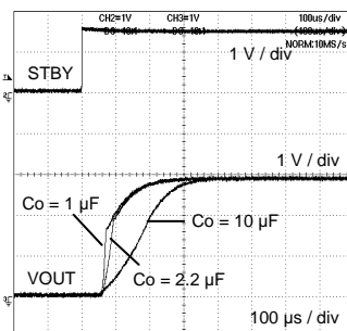
Fig.23 Output Voltage Rise Time (BH30NB1WHFV)
