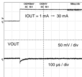
Fig.19 Load Response (Co = 2.2 µF) (BH25NB1WHFV)
