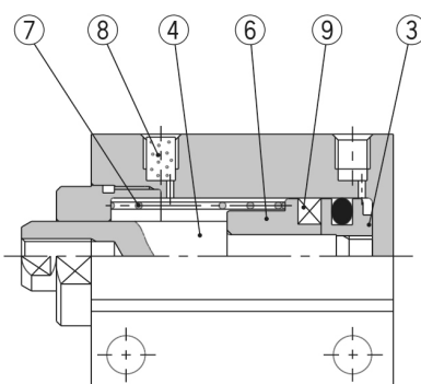
Built-in magnet
